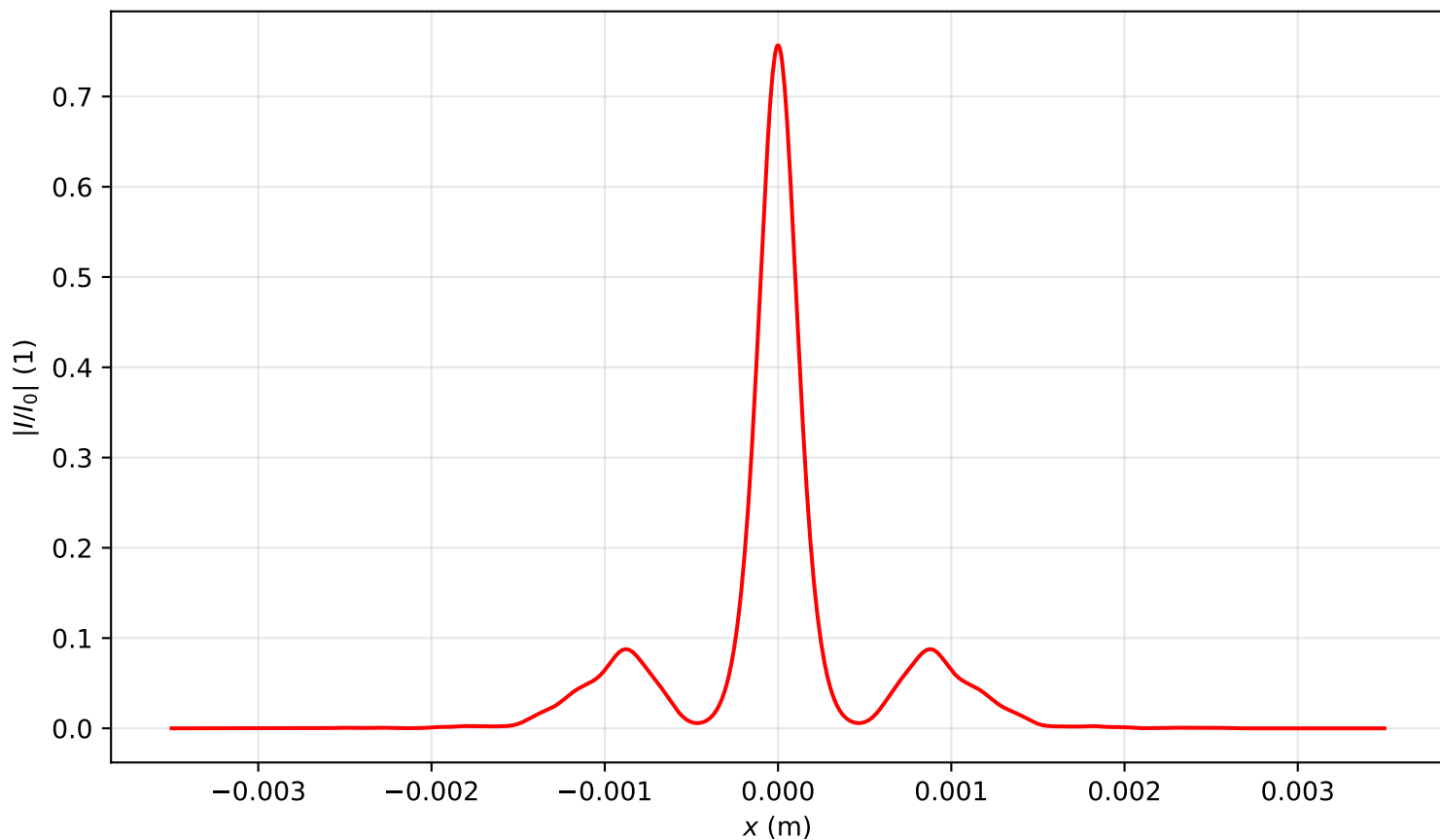
Intensity profile I(x, y = 0, z = 2.149)/I_0 , P_{in}=8.5P_{cr} , artificial time
